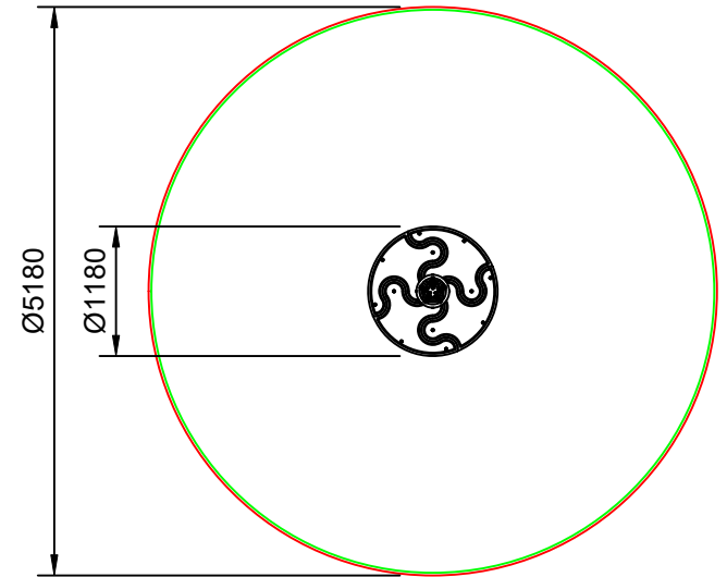
Plan View Scale: 1:75
